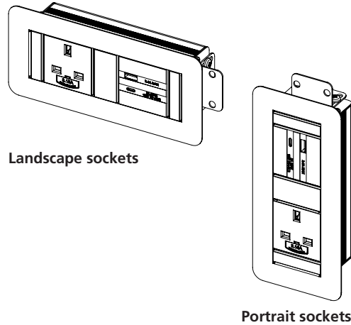
Portrait sockets
